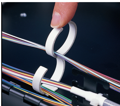
SWIC3-M, SWIC3 Dual-Level Fiber Managers incorporate two independent levels of storage to enable fiber to be routed at levels that correspond to the adapters
